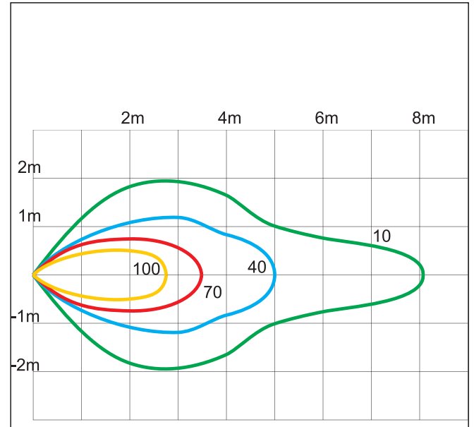
Vertical sensitive area
