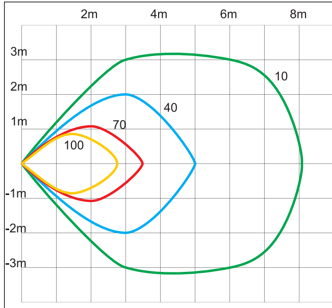
Horizontal sensitive area
